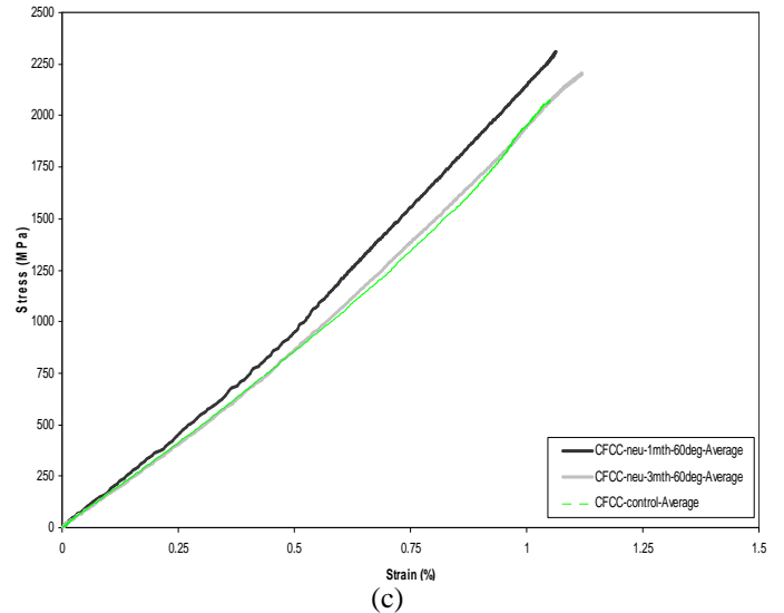
Figure 8: Unstressed stress-strain relationships of steel and CFCC strand over 0, 1 and 3 months curing in various aggressive solutions at a curing temperature of 60°C (a) CFCC curing in alkaline groundwater, (b) CFCC curing in acidic groundwater and (c) CFCC curing in neutral solution.
