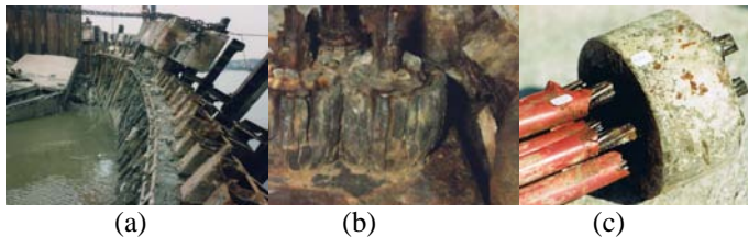
Figure 2: Failure of anchored quay wall (a) corroded barrels and wedges in anchor head (b) lack of corrosion protection behind anchor block [8]
