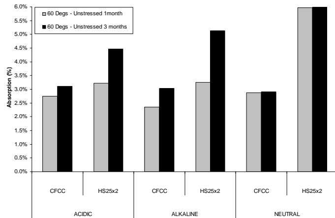
Figure 5: Absorption of specimens immersed in aggressive groundwater at elevated temperatures
