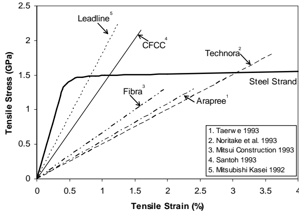
Figure 3: Typical tensile stress-strain behaviour of various FRP products compared to steel strand [after 2]
