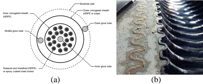
Figure 1: (a) Schematic of double protection system for permanent ground anchor; (b) longitudinal section - double corrosion protection through the bond length of a ground anchor [8].
