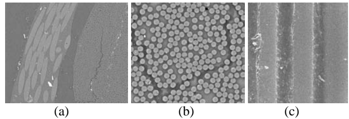
Figure 7: SEM analysis on CFRP strand prior to immersion into aggressive groundwater solution (a) CFCC at 100x magnification (b) CFCC at 500x magnification (c) HS25x2 at 1000x magnification
