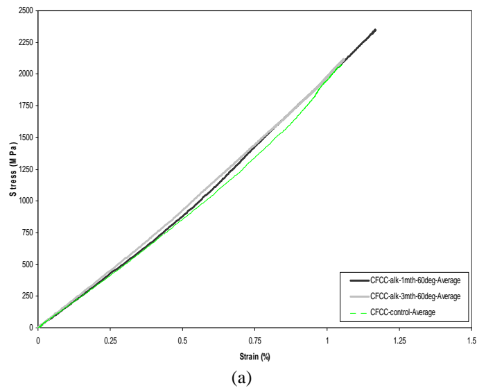
Figure 8: Unstressed stress-strain relationships of steel and CFCC strand over 0, 1 and 3 months curing in various aggressive solutions at a curing temperature of 60°C (a) CFCC curing in alkaline groundwater, (b) CFCC curing in acidic groundwater and (c) CFCC curing in neutral solution.
